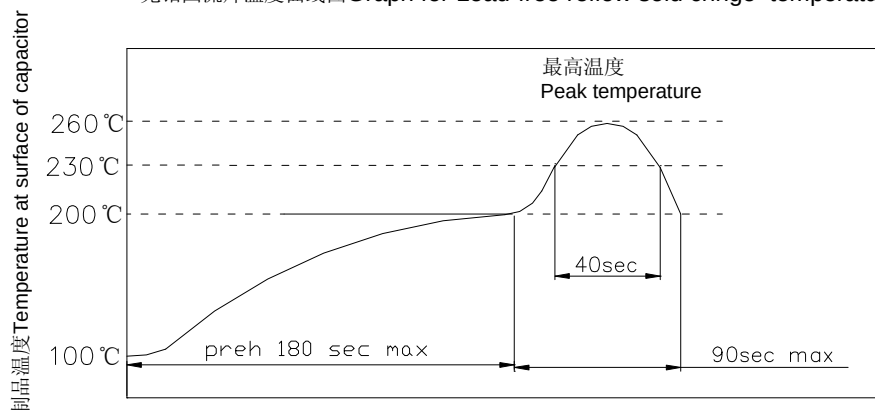
无铅回流焊温度曲线图 Graph for Lead-free reflow soldering temperature
